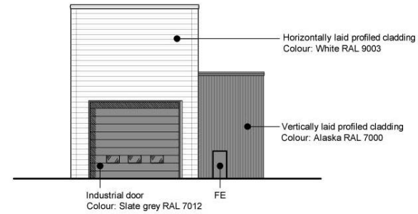
Wood Store East Elevation
