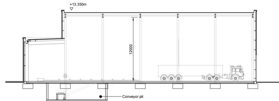
Wood Store Section
