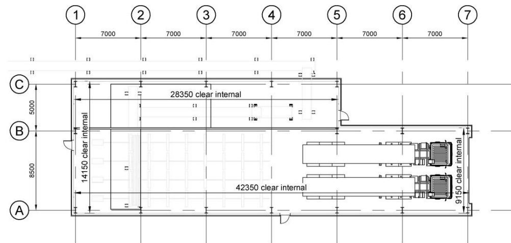
Wood Store Layout
