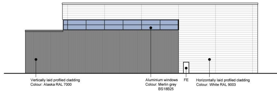
Wood Store South Elevation
