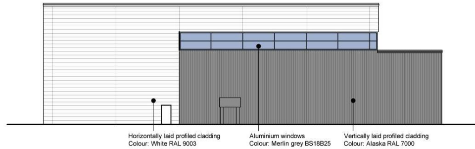
Wood Store North Elevation
