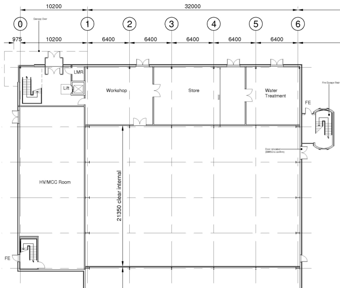
Offices, Workshop, Stores & Plant Ground Floor Layout
