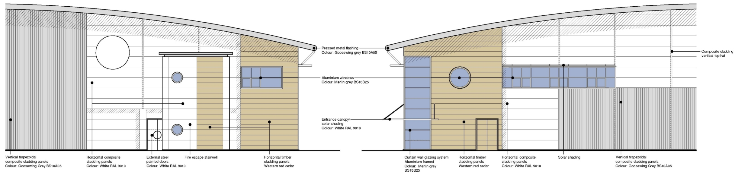
Offices, Workshop, Stores & Plant East Elevation
