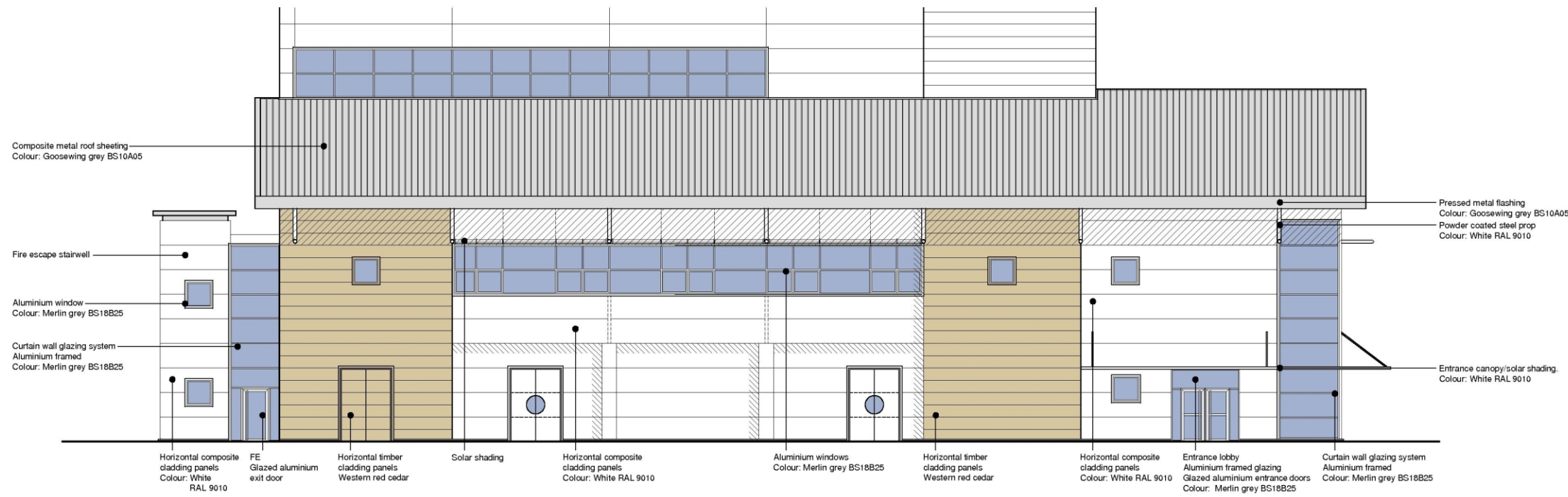
Offices, Workshop, Stores & Plant North Elevation
