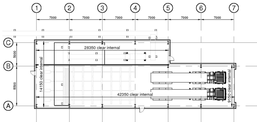
Wood Store Layout
