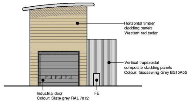
Wood Store East Elevation
