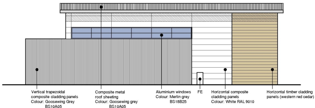
Wood Store South Elevation
