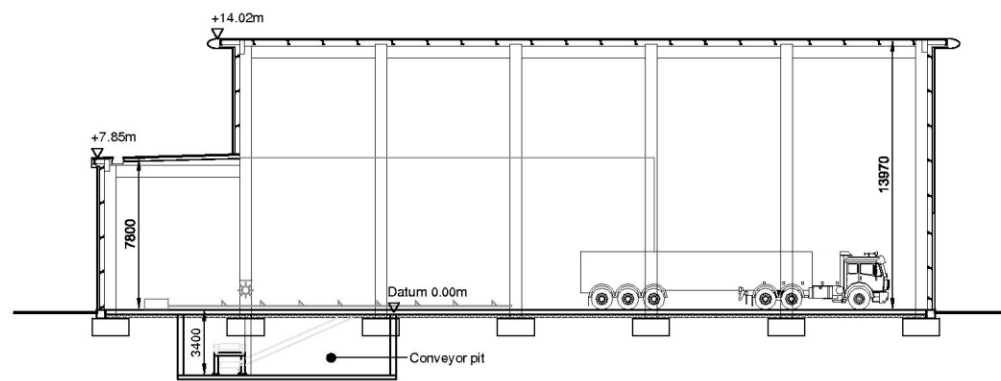
Wood Store Section
