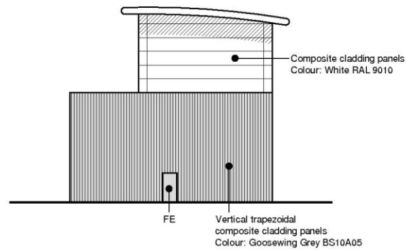
Wood Store West Elevation
