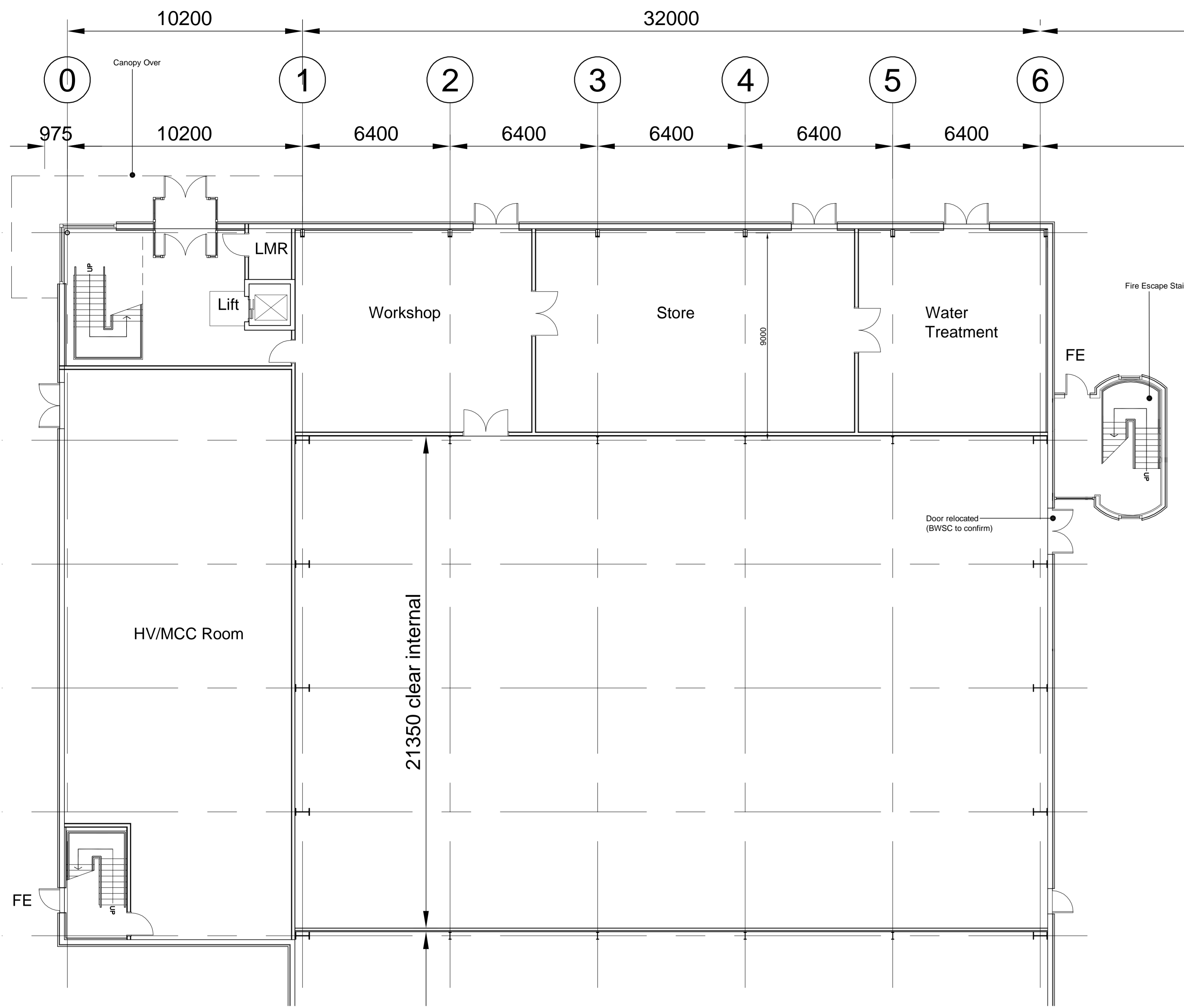
Offices, Workshop, Stores & Plant Ground Floor Layout
