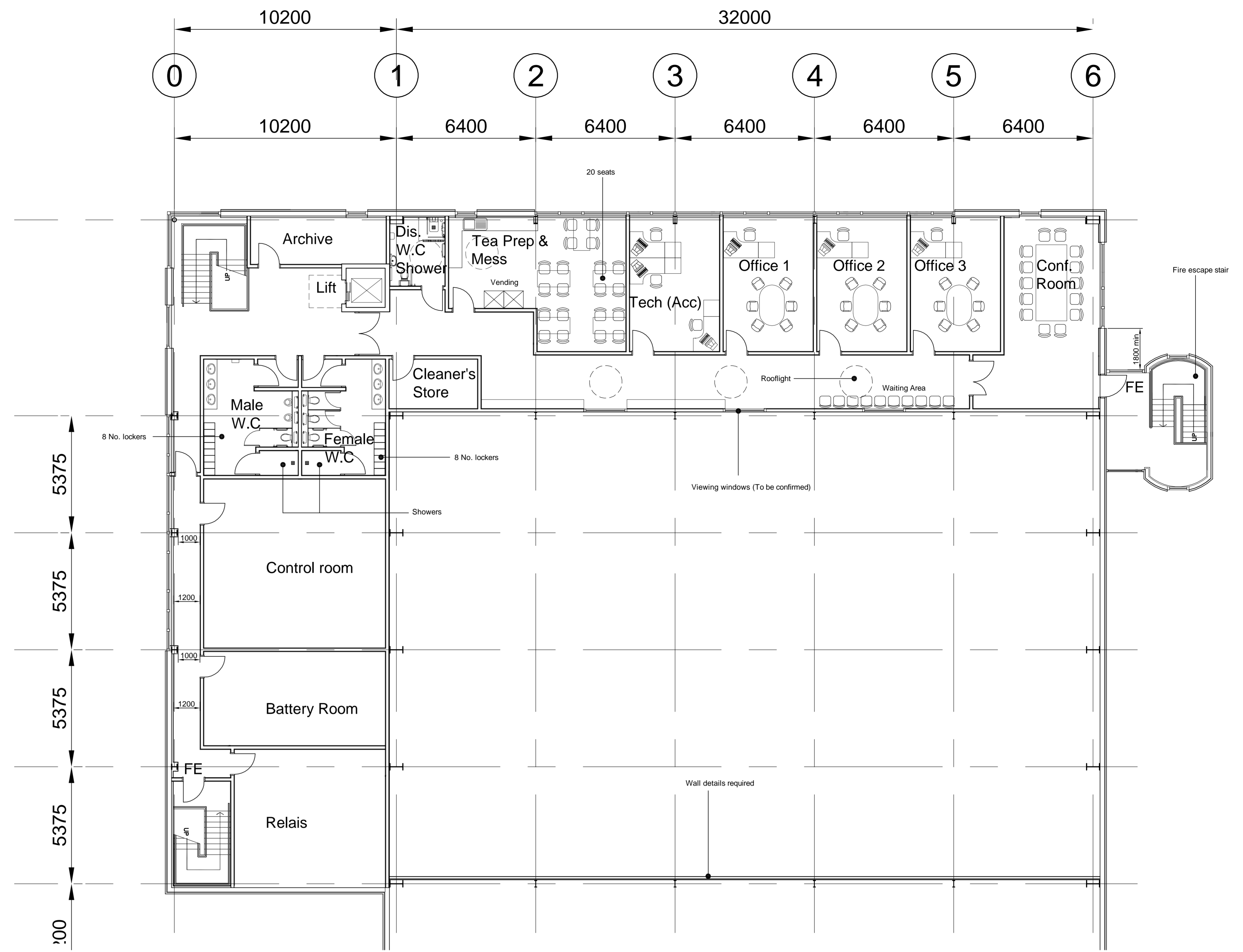
Offices, Workshop, Stores & Plant First Floor Layout
